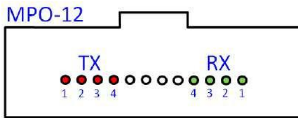
Figure 2 – Active fiber ports in MPO12 connector on module side
