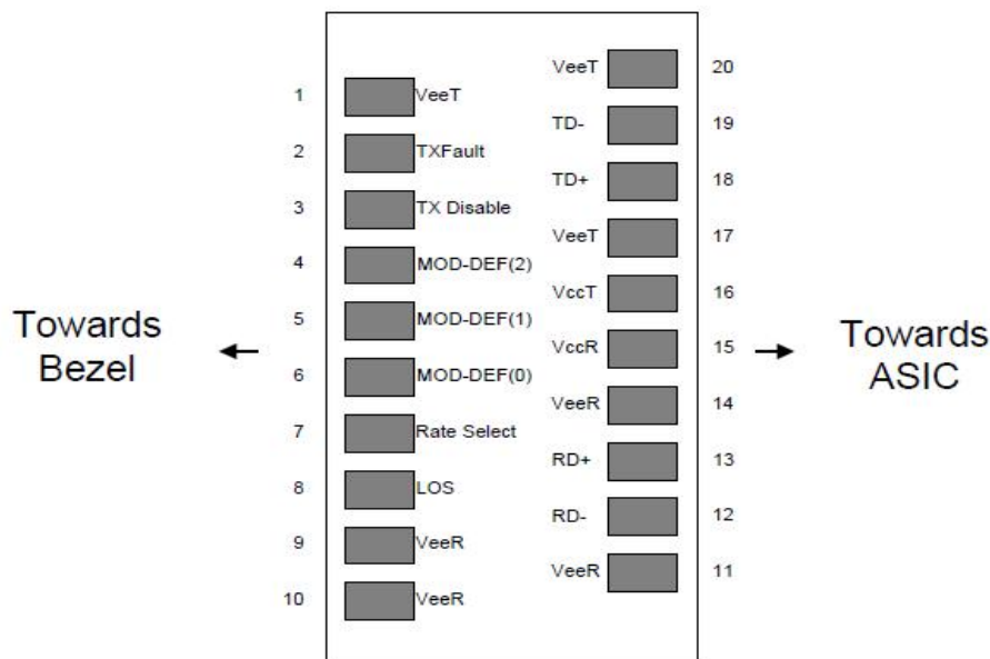
Figure 2: Pin-out of Connector Block on Host Board
