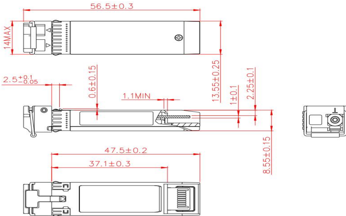
Figure 3. Module Mechanical Dimensions
