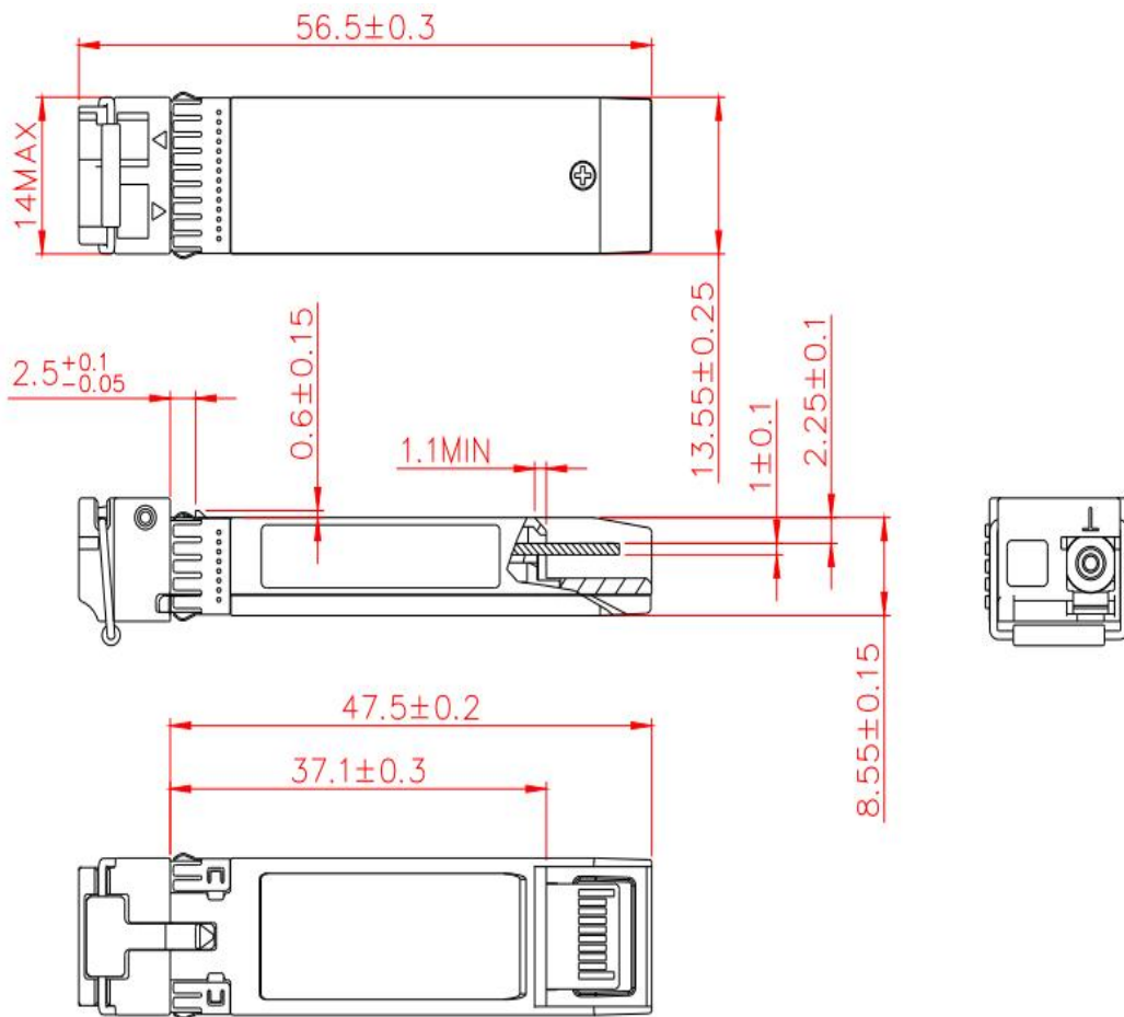
Figure 3. Module Mechanical Dimensions
