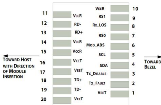
Figure 1.Pin function definitions
