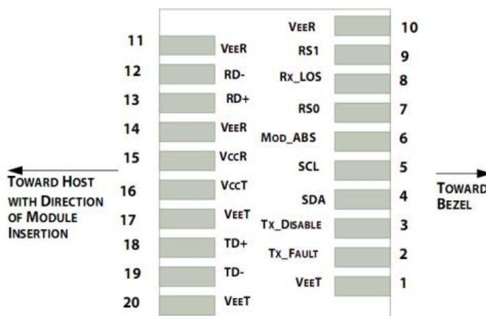
Figure 1.Pin function definitions
