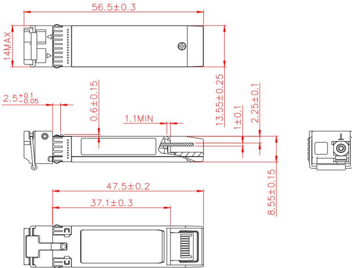
Figure 3. Module Mechanical Dimensions
