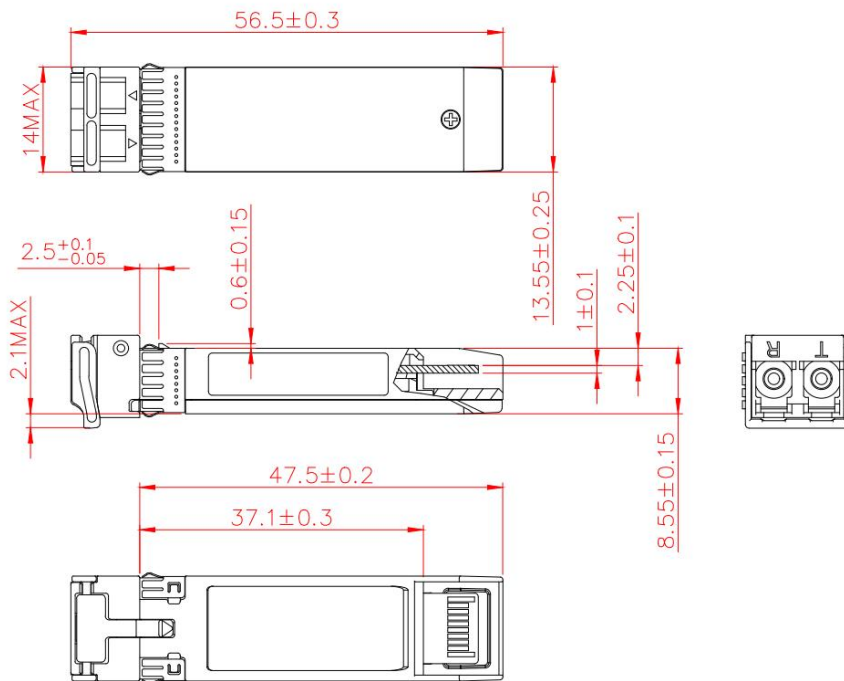
Figure 3. Module Mechanical Dimensions
