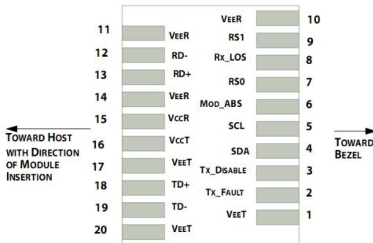
Figure 1.Pin function definitions
