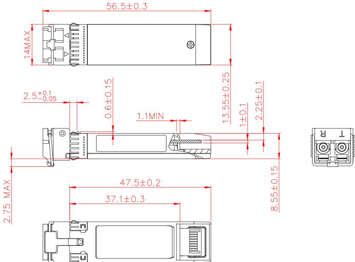
Figure 3. Module Mechanical Dimensions
